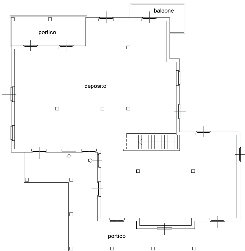
PIANO TERRA - h = 2,70 m.
